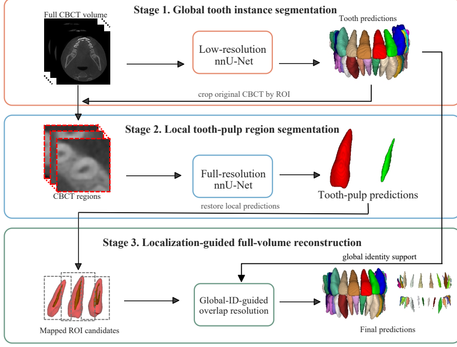
Fig. 1. Overview of the proposed two-model, three-stage global-to-local framework. A low-resolution nnU-Net predicts global tooth instances and constructs tooth-wise ROIs, a shared full-resolution nnU-Net segments the tooth and pulp regions within each ROI, and the mapped local predictions are reconstructed in the original CBCT space using the global tooth identities.
